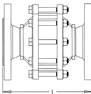
Flanged connection
